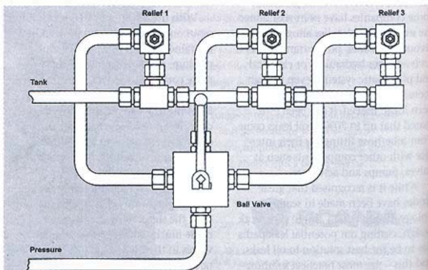
FIGURE 3: Line-mounted circuit
